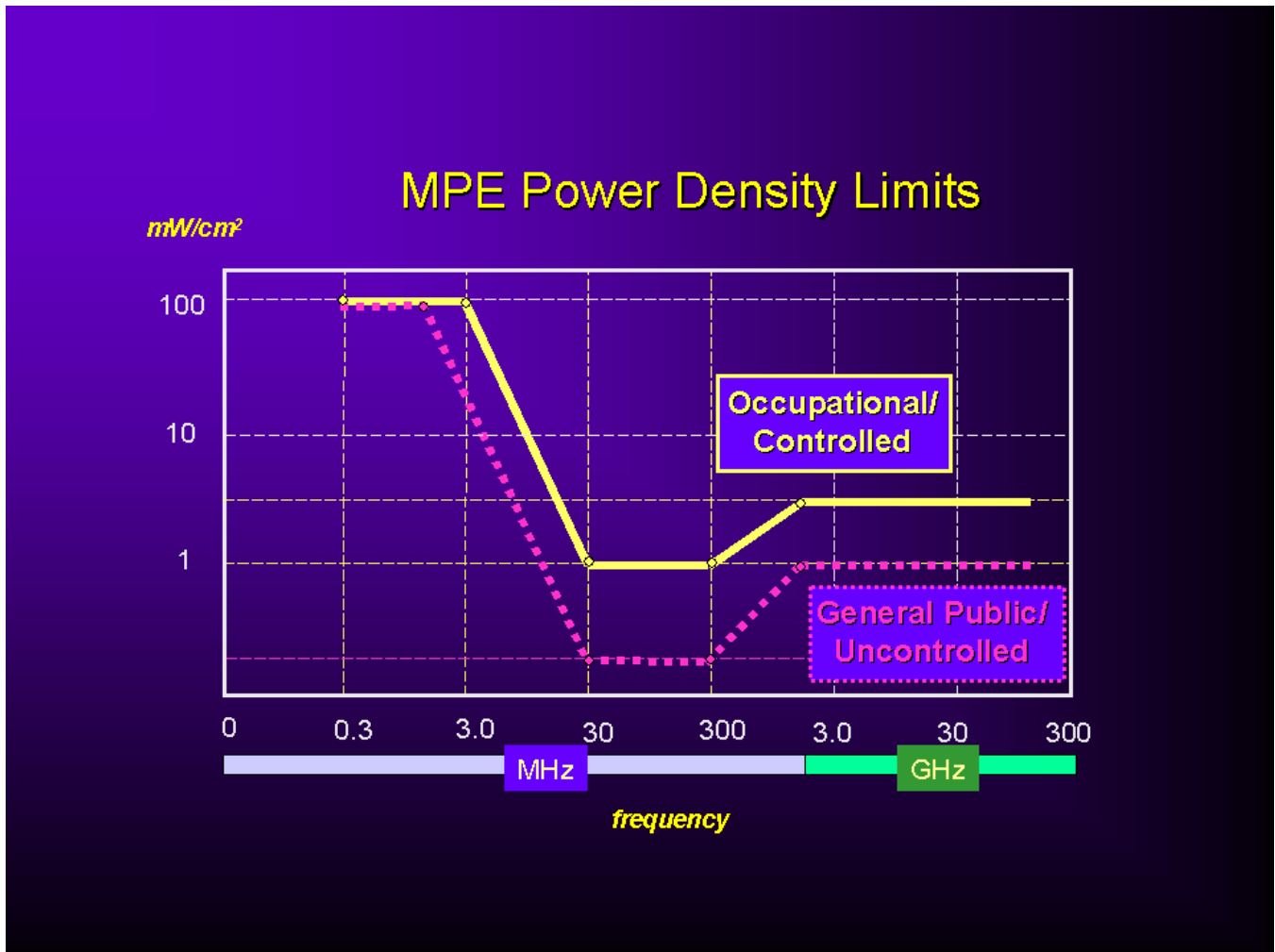
Power Density Curve as defined in OET 65
